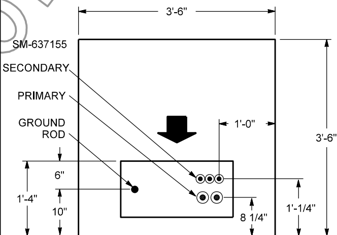
STUB-UP LOCATION DETAIL
