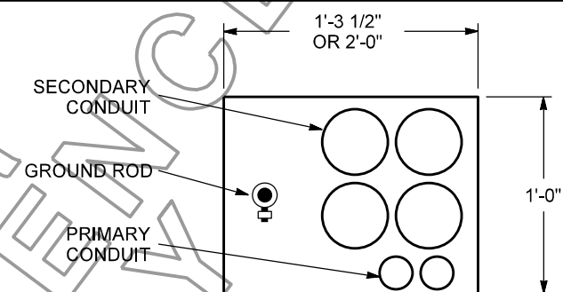
CONDUIT STUB-UP DETAIL 1Φ TRANSFORMER WINDOW FOR MORE THAN FOUR (4) SECONDARY CONDUITS, USE J-BOX PER SEPARATE DETAIL.
