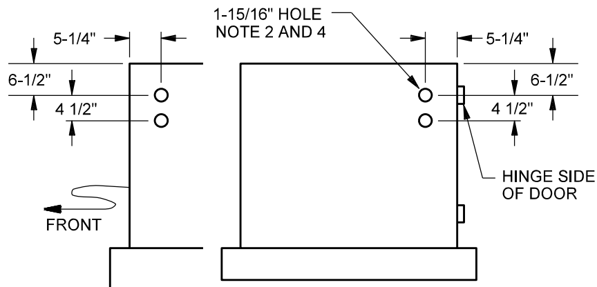
FRONT VIEW OF SWITCH
