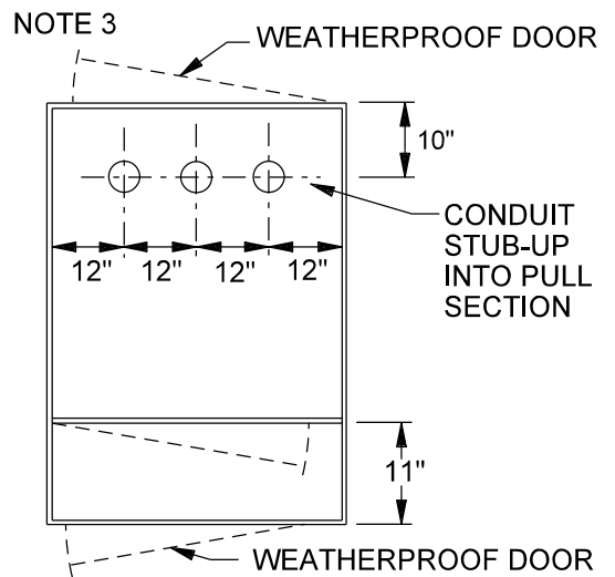
BASE PLAN
