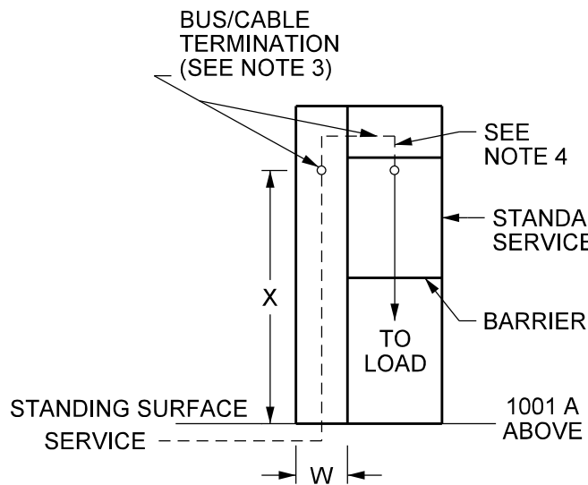
FIG.1 SWITCHBOARD PULL SECTION
