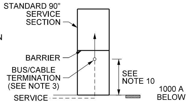
FIG.2 BOTTOM FEED 400-1000 AMPS
