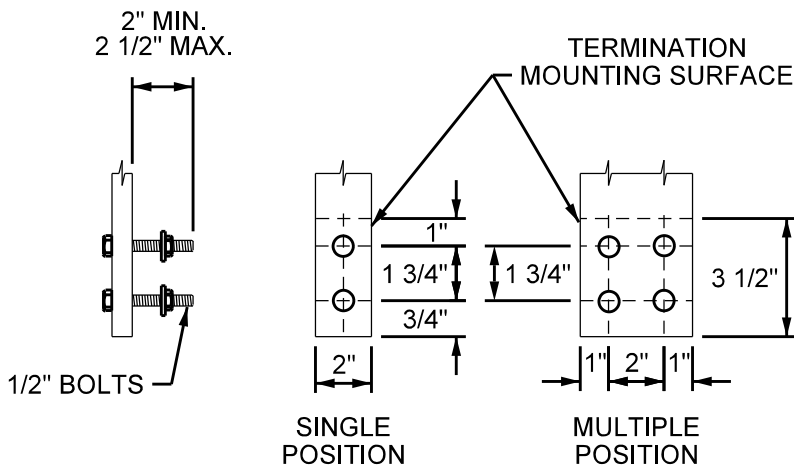
FIG. 1 TERMINATING BOLT AND DRILLING DETAIL OF TERMINATING FACILITIES
