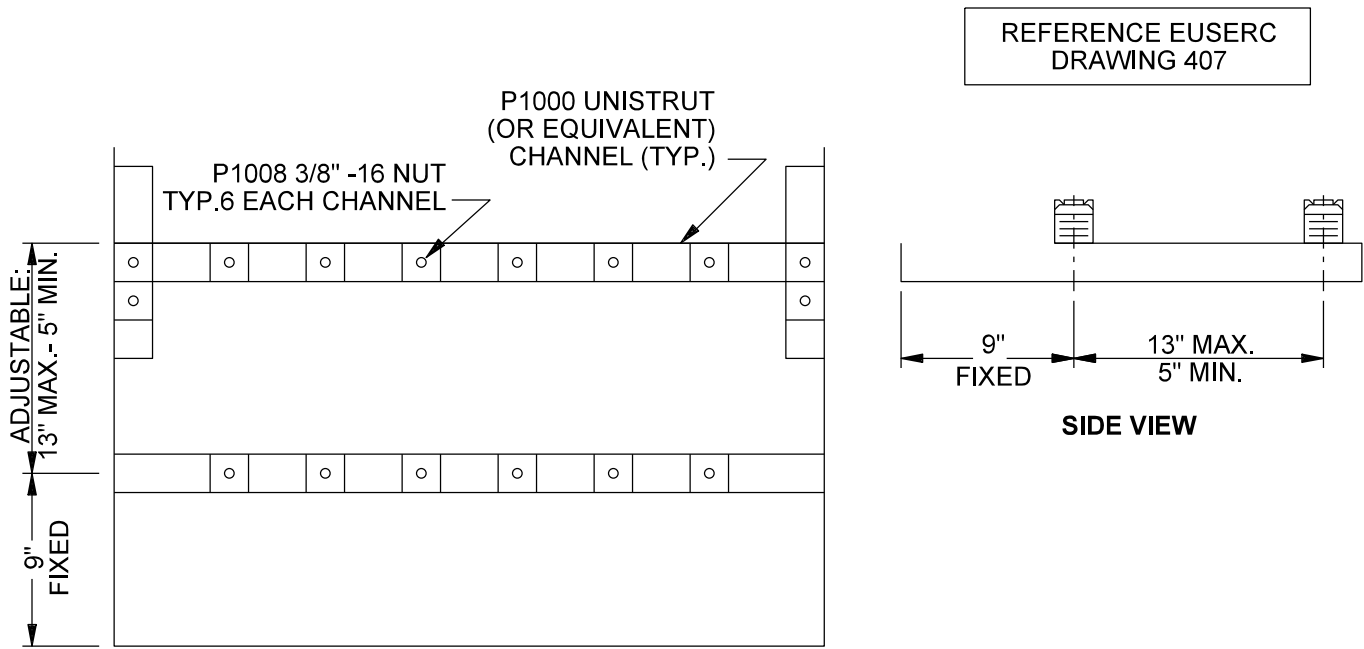
TOP VIEW OF CABINET (REF.)
