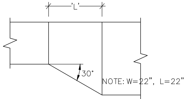
ECCENTRIC TRANSITION
