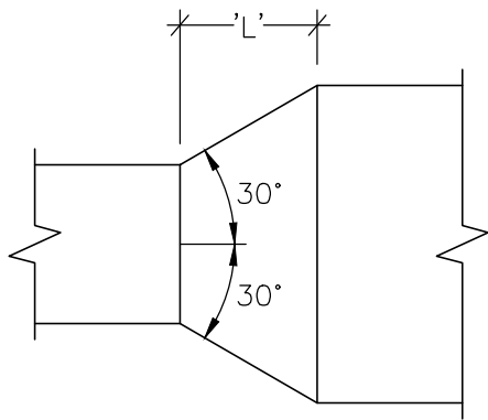
CONCENTRIC TRANSITION
